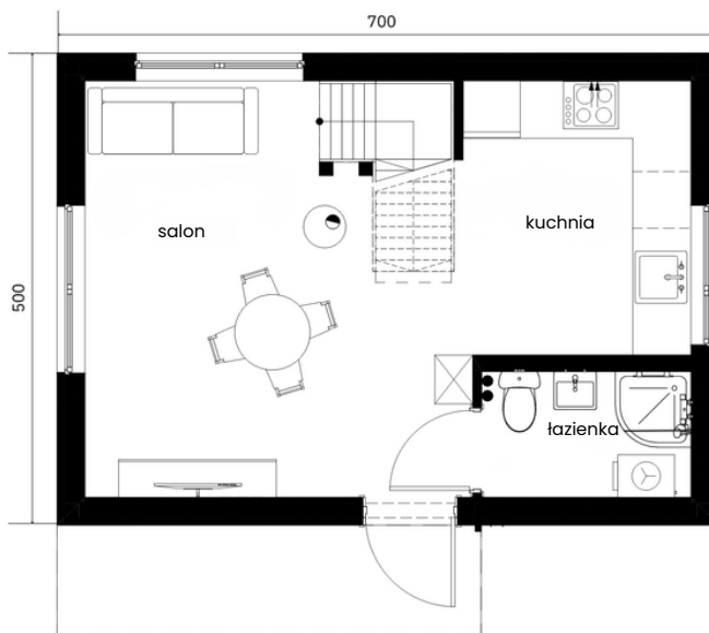
parter
